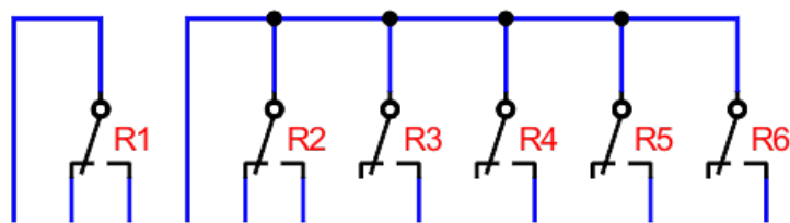
Figure 1: Relay configuration
